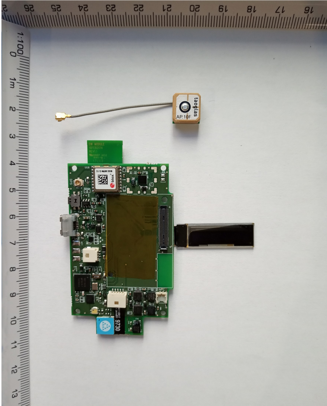
Photo 3: WIMU PRO – PCB side 1 and GNSS antenna.
